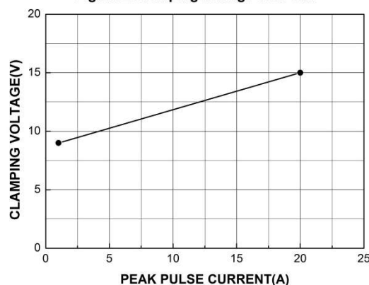
Figure 2 Clamping Voltage Vs. Peak
