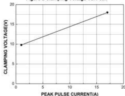
Figure 2 Clamping Voltage Vs. Peak
