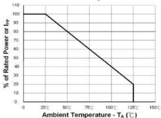
Power Derating
