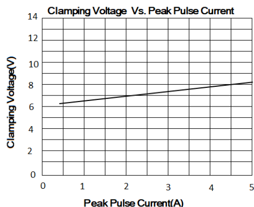
Positive TLP Clamping Voltage (tperiod=100ns, tr=1ns)
