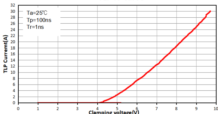
TLP IV curve
