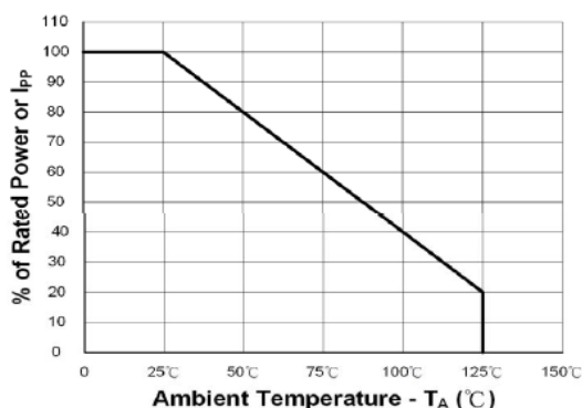
Figure 1. Power Detating
