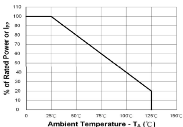
Figure 1. Power Detating
